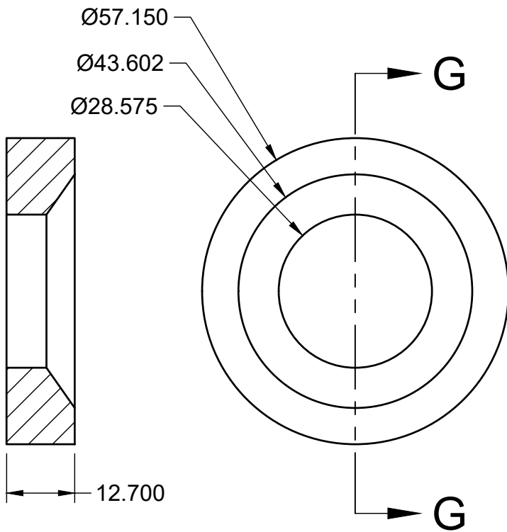
SECTION G-G
