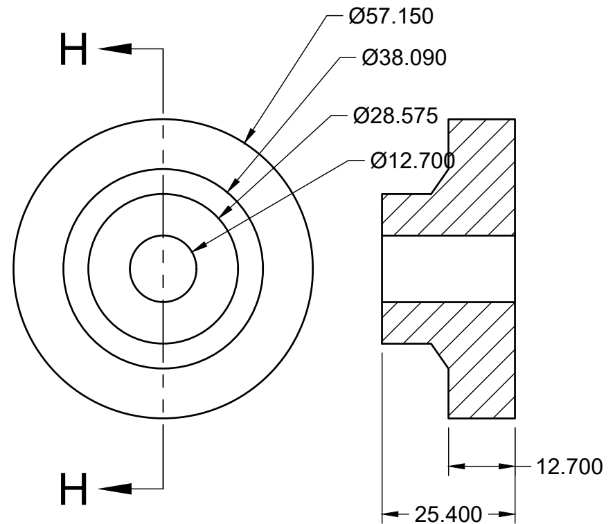
SECTION H-H
