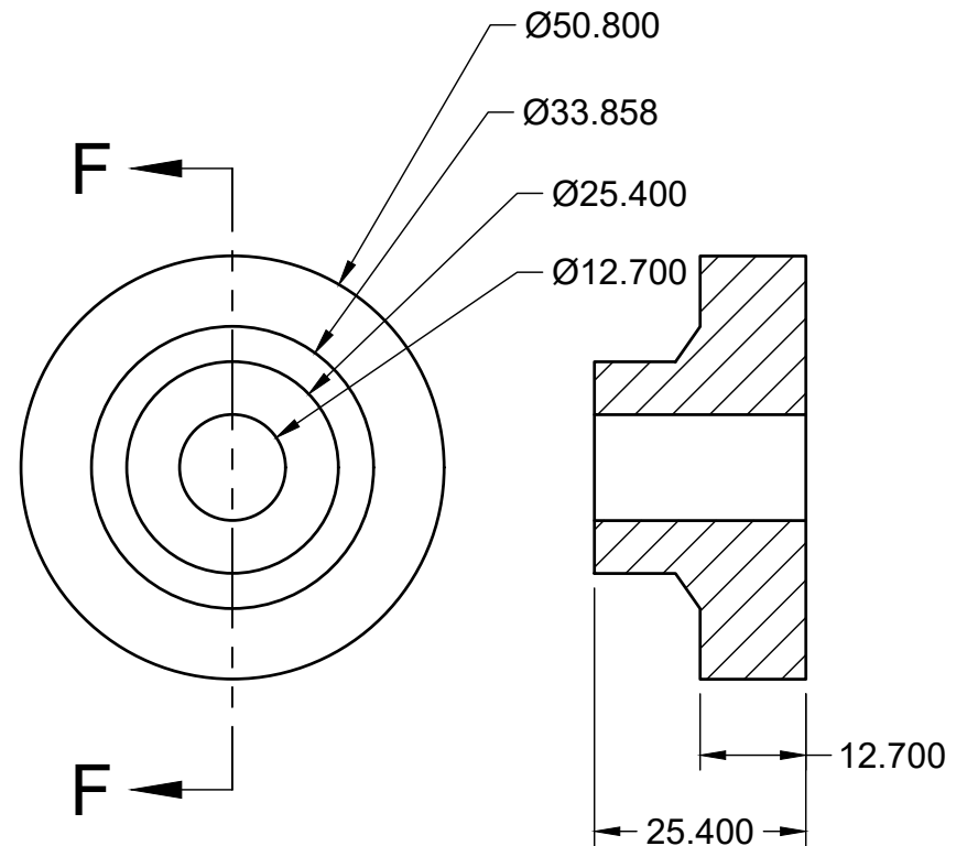
SECTION F-F
