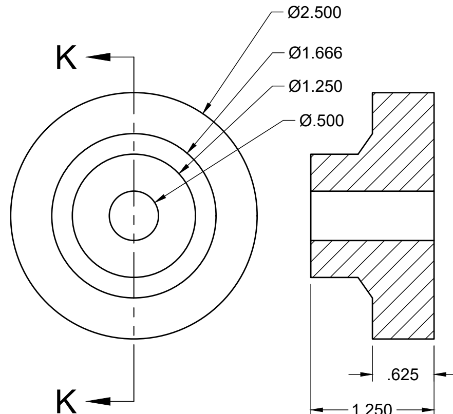
SECTION K-K
