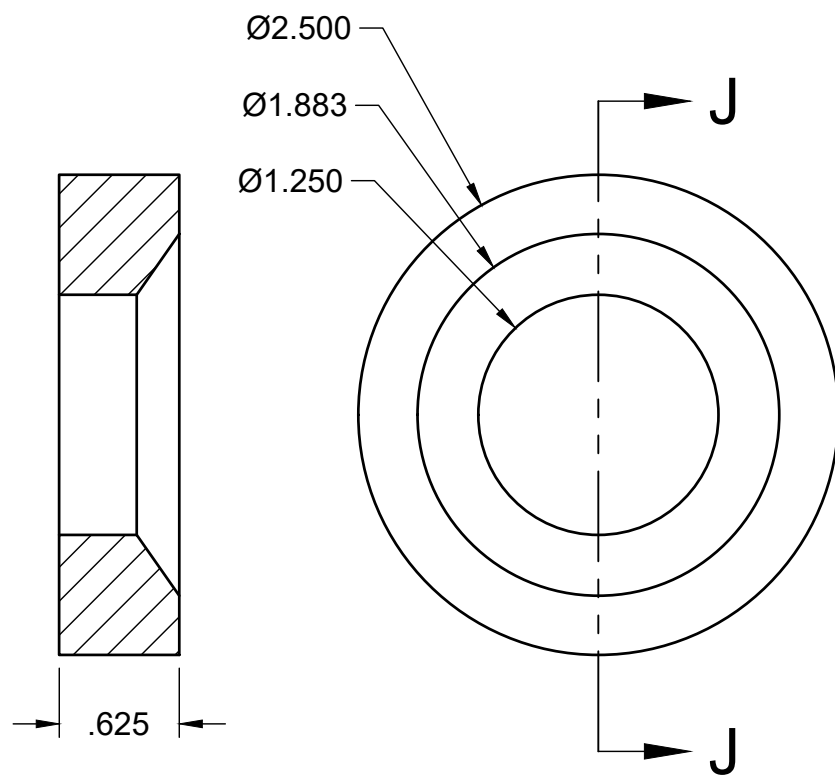
SECTION J-J
